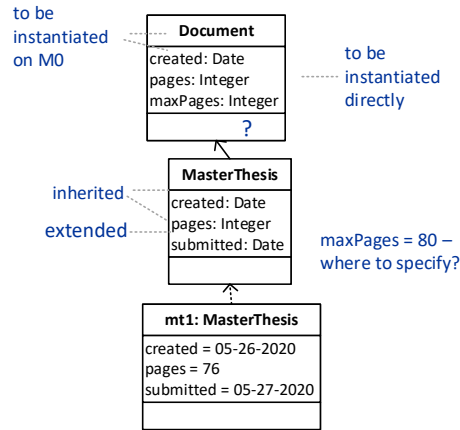
Fig. 1. Illustration of limited expressiveness in traditional paradigm
