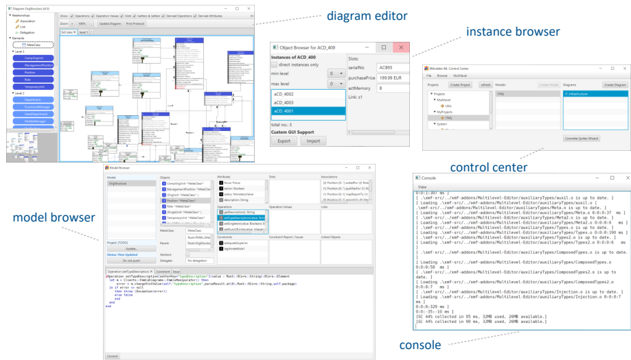
Fig. 6. Components of the XModeler ML
