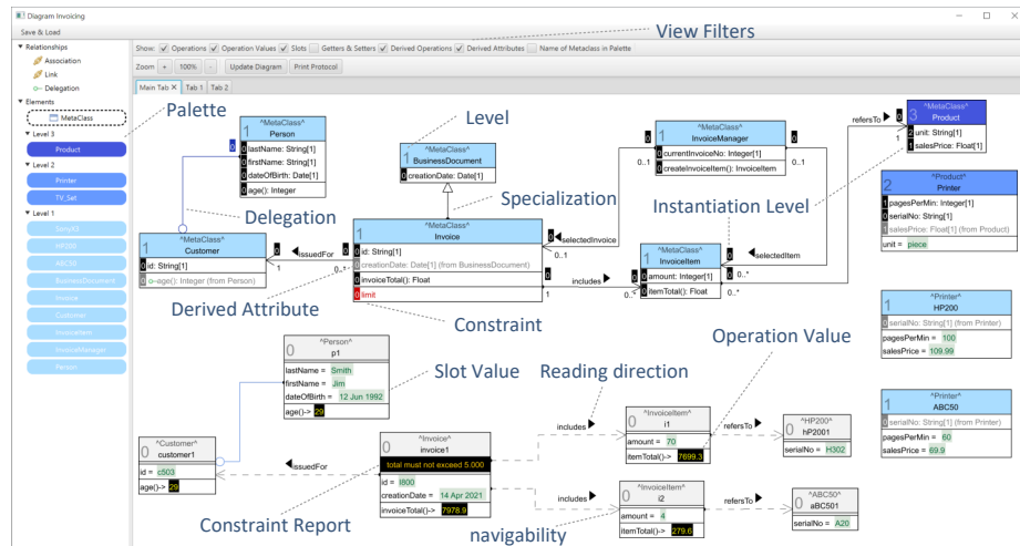
Fig. 5. Illustration of concepts provided by the FMML x
