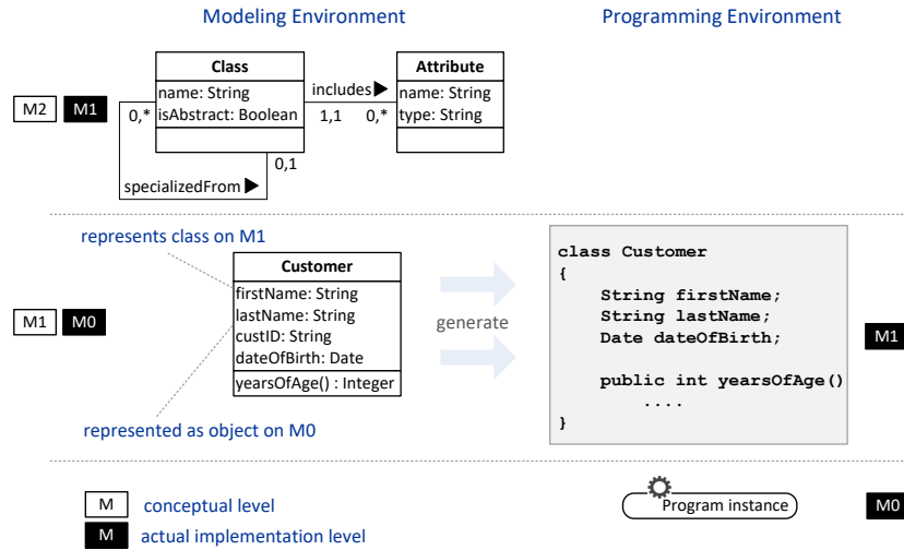
Fig. 2. The reason for software generation
