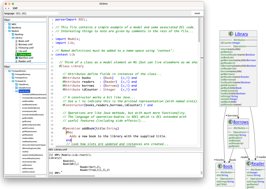
Fig. 4. A Simple Executable Model in XEditor and Associated Diagram
